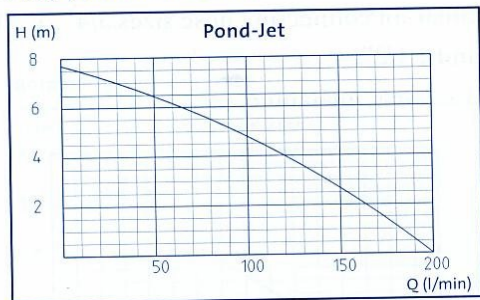
Comparison of pump performance curves, s. p. 132 – 135.
